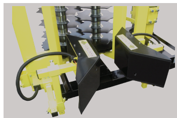
Magnetic sensors - open and close cutting heads when sensing steel posts
